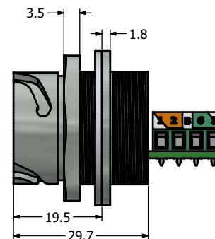
Panel Nut (M28 x 1.5)
